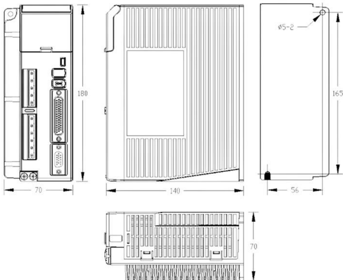
Driver Leadshine H2-2206
